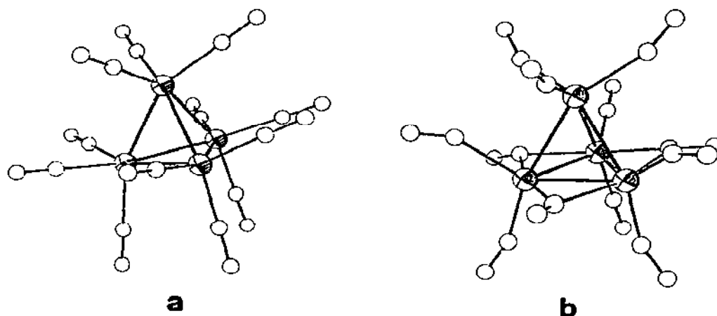
Fig. 8. (a) Molecular structure of \text{Ir}_4(\text{CO})_{12}(\text{TJ}) . (b) Molecular structure of \text{Co}_4(\text{CO})_{12}(\text{C}_{3v}) .
